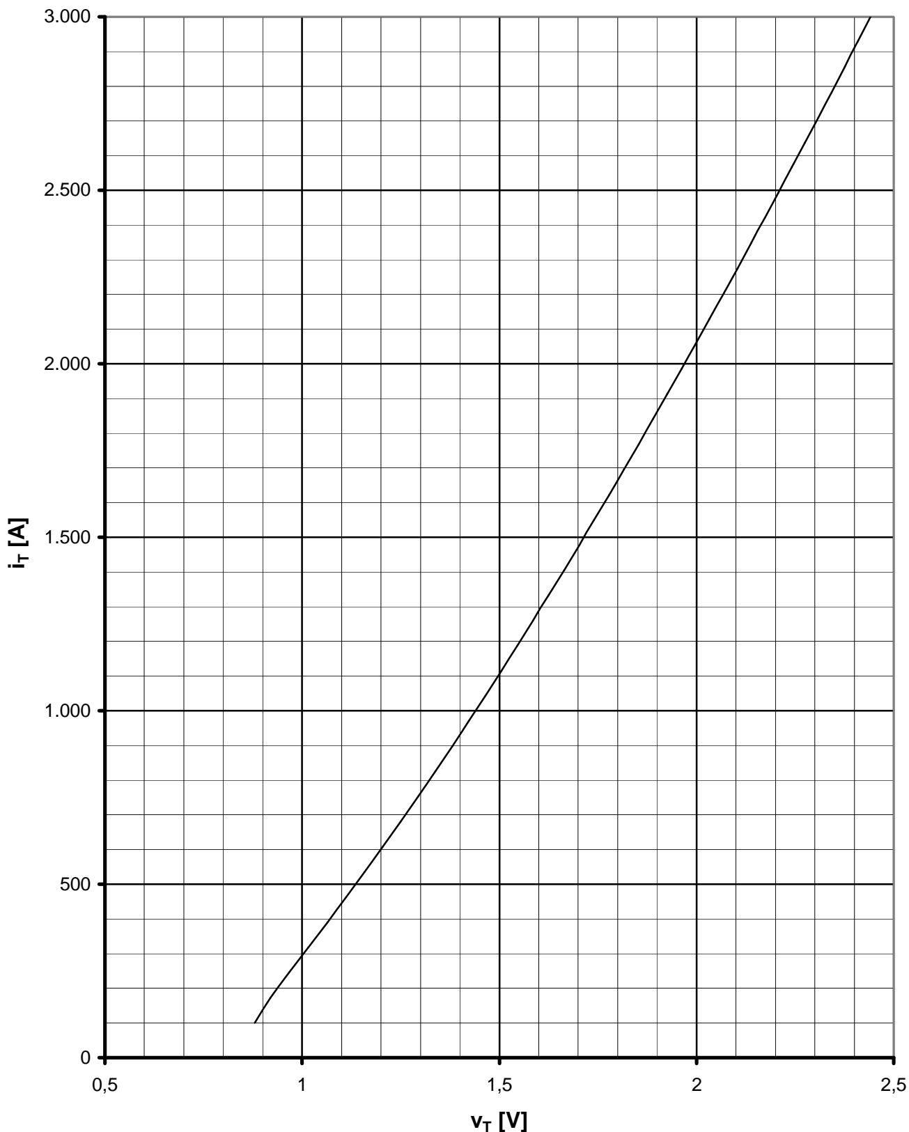
Grenzdurchlaßkennlinie / Limiting On-state characteristic i_T = f(v_T)
